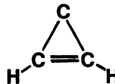
Figure 3. Cyclopropenylidene molecule.
